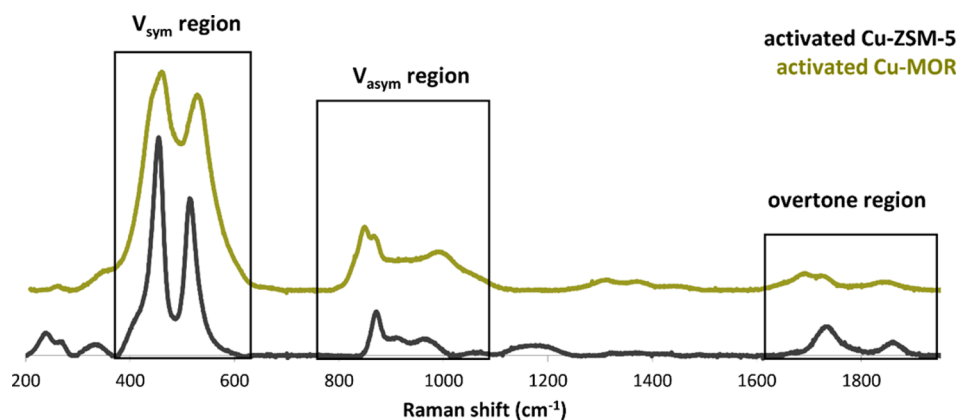
Figure 5. Comparison of the resonance Raman spectra ( \lambda_{\text{ex}} = 458 \text{ nm} ) of \text{O}_2 activated Cu-MOR and Cu-ZSM-5.
